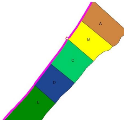
Figure 7: Gaza coastal zone classified into five regions according to Rate of coastal change
