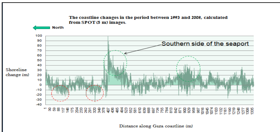
Figure 8: Rate of coastal change along Gaza coastline
