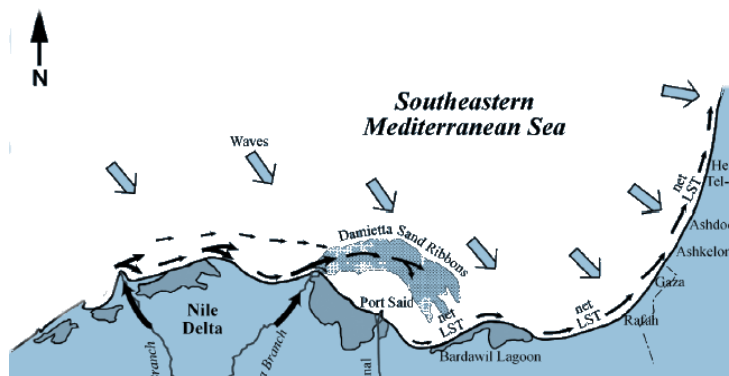
Figure 2: Longshore sediments transport along the South-eastern Mediterranean Coast, (Zviely, 2006)
