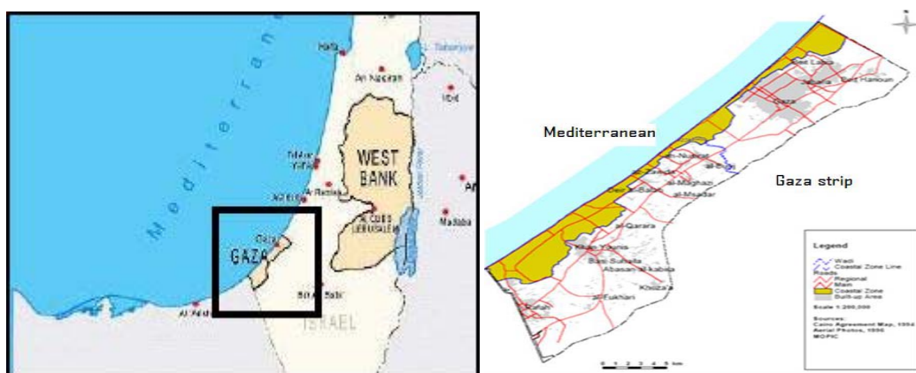
Figure 1: Location of Gaza Strip on the Levantine Basin (left) and the coastal zone of Gaza Strip (right). (Gaza Coastal and Marine Environmental Action Program, Ministry of Environmental Affairs, 2000)
