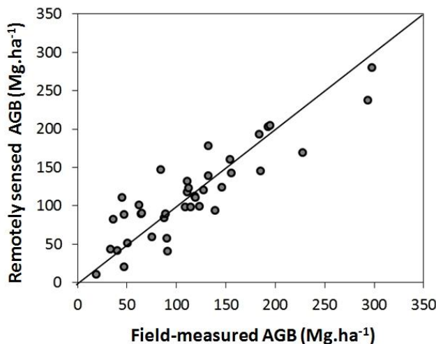
Figure 2. Scatterplot of field-measured biomass for the plots established during the forest inventory (x axis) versus the remotely sensed biomass (y axis) as calculated from the best model. Source: adapted from [29].
